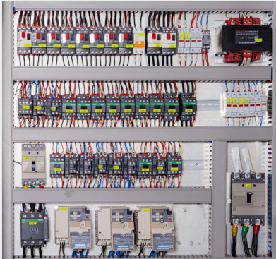
● 电器箱 Electrical cabinet
